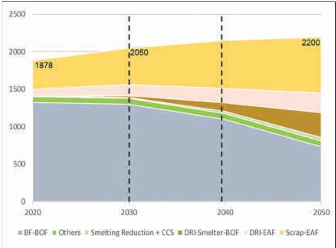
Fig 3 Primetals Technologies forecast of the shift to DR, EAF and smelter routes
