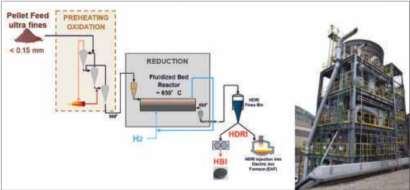
Fig 2 HYFOR process flow sheet (L) and the pilot plant installation (R)
