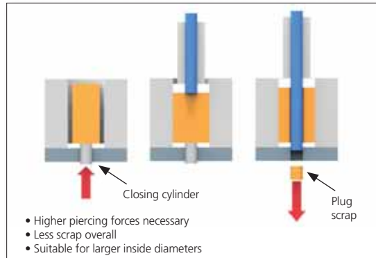
Ⓐ Fig 4 Piercing with prior upsetting
