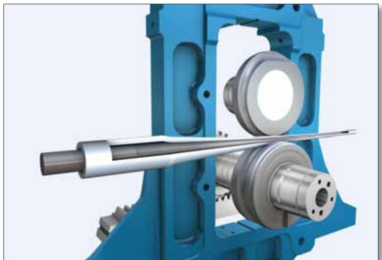
ⓐ Fig 8 Principle of the cold pilgering process
