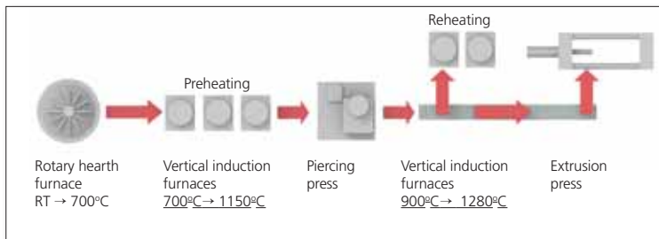
Fig 2 Heating concept
