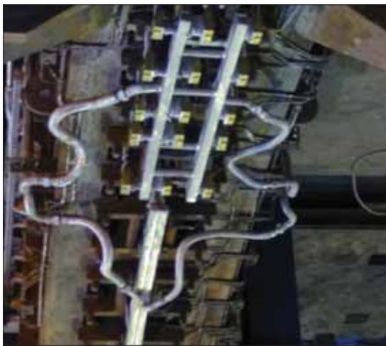
Fig 6 Segments 1 & 2 with new air-mist headers mounted on strand 1 during cold commissioning
